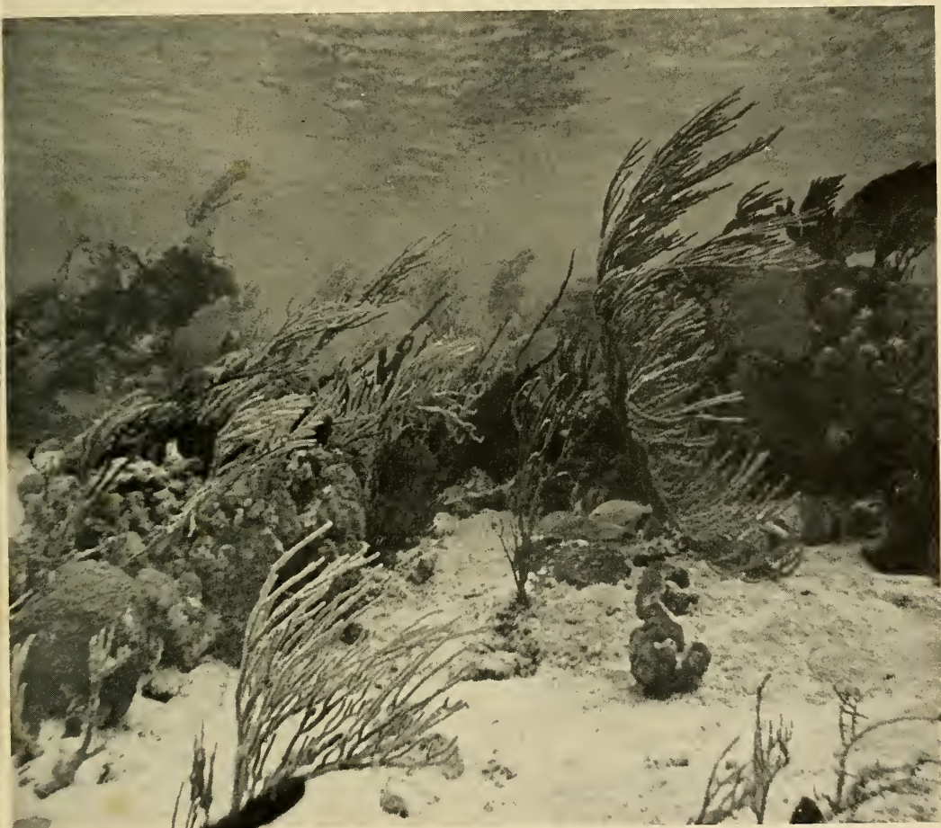
GORGONIAS AND SPONGE AT TWELVE FOOT DEPTH
