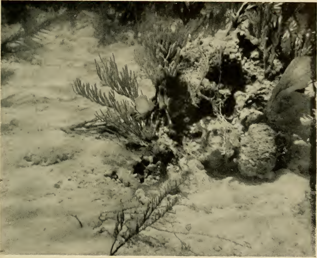
AN EXAMPLE OF NATURE'S ARTISTRY
